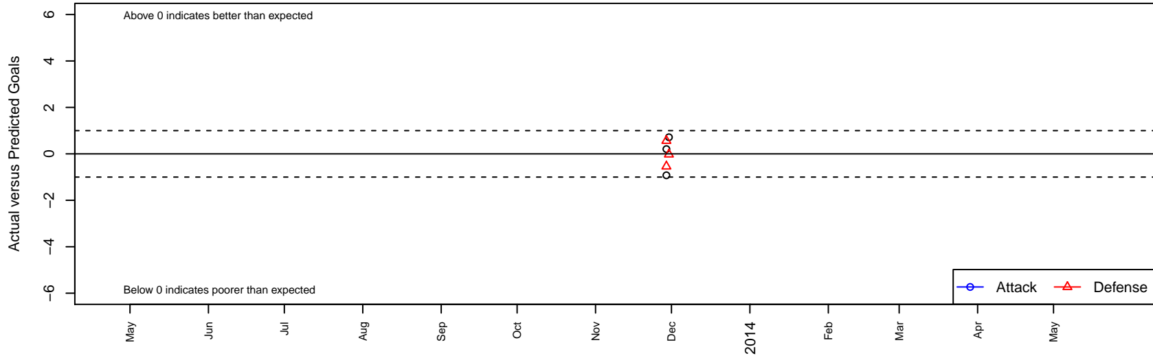
Select Cities SC Avalanche G99 Dots are actual minus expected GF (blue circles) and GA (red triangles). Blue line is smoothed change in attack strength. Red is smoothed change in defense strength.
